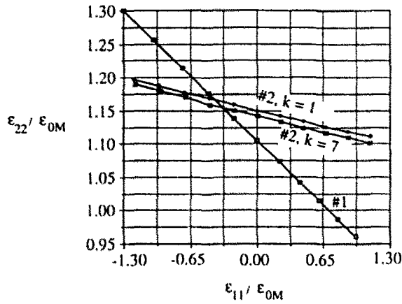
Fig. 11. Strains at localization for model No. 1 and model No. 2 when \alpha ranges from -1 to +1 .
